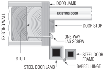
INSET MOUNT W/TAB
