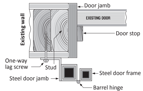
Surface mount w/stand-off tabs
