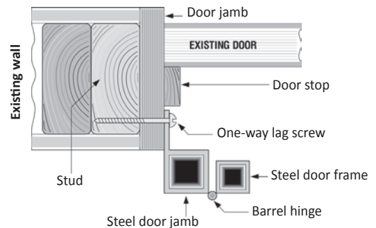
Inset mount w/tab
