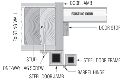
SURFACE MOUNT W/TABS
