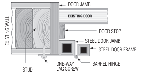
INSET MOUNT W/SURFACE TABS
