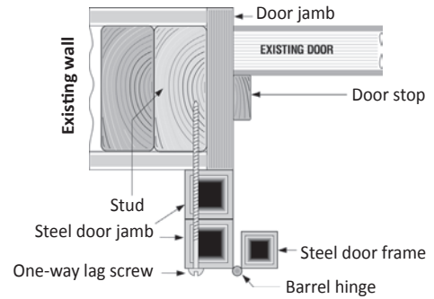
Surface mount w/tube backing
